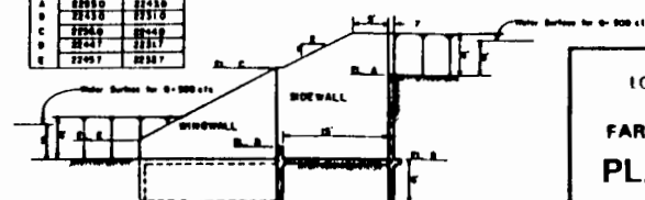
DETAIL C DROP STRUCTURE AT STATIONS 85+30 & 80+20 NO SCALE
