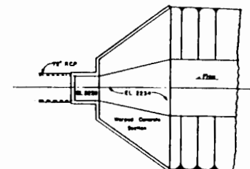
DETAIL B PLAN OF NEW INTAKE STRUCTURE AT STATION 129+35 SCALE IN FEET 0 10 20
