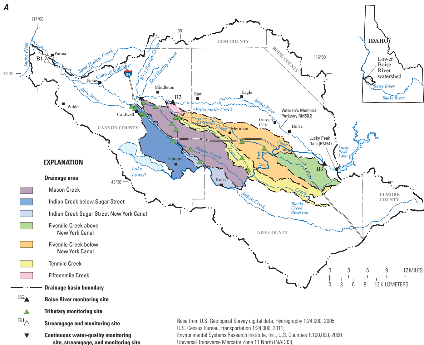
Figure 1. Locations of water-quality, biological, and bottom-sediment sampling sites in the (A) study area and (B) Mason, Indian, Fivemile, and Tenmile Creeks, and (C) land use changes between 1992 and 2006, lower Boise River watershed, southwestern Idaho.
