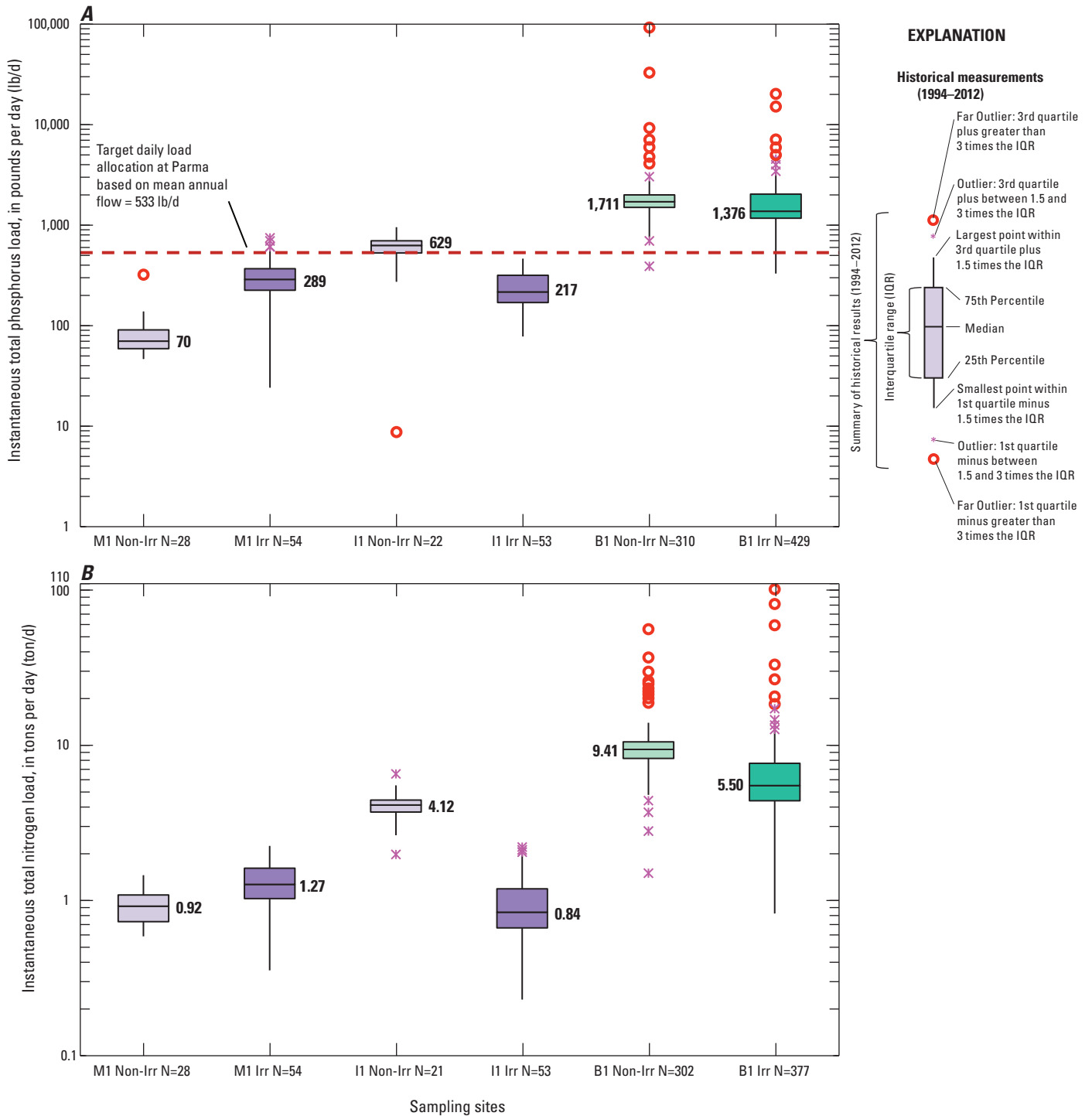
Figure 9. Historical instantaneous (A) total phosphorus and (B) total nitrogen loads in irrigation and non-irrigation seasons in Mason and Indian Creeks (sites M1 and I1) (1994–2012) and the Boise River near Parma (site B1) (1969–2012), southwestern Idaho. Locations of sites are shown in figure 1B . (N, number of samples).
