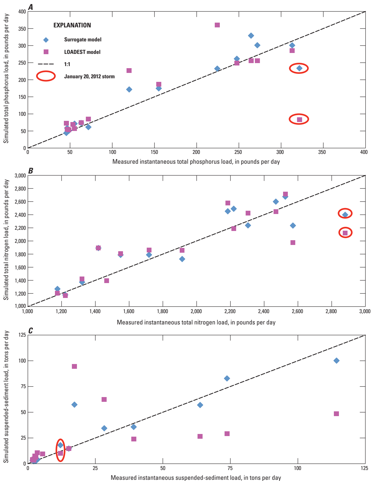
Figure 19. Measured instantaneous loads of (A) total phosphorus, (B) total nitrogen, and (C) suspended sediment compared with estimated loads using U.S. Geological Survey LOAD ESTimator (LOADEST) and surrogate models, Mason Creek near Caldwell (site M1), Idaho, March 2011–March 2012.
