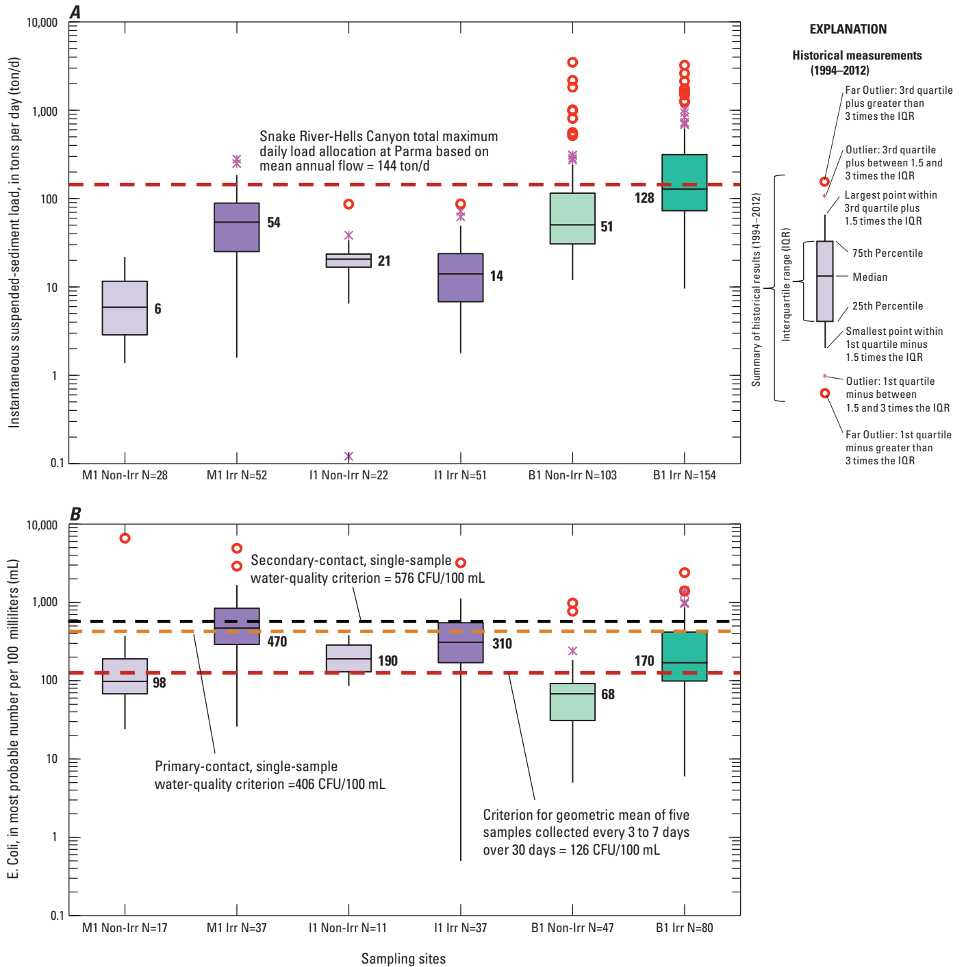
Figure 11. Historical instantaneous (A) suspended-sediment loads and (B) Escherichia coli ( E. coli ) values in irrigation and non-irrigation seasons in Mason and Indian Creeks (sites M1 and I1) (1994–2012) and the Boise River near Parma (site B1) (1969–2012), southwestern Idaho. Locations of sites are shown in figure 1B . (N, number of samples).
