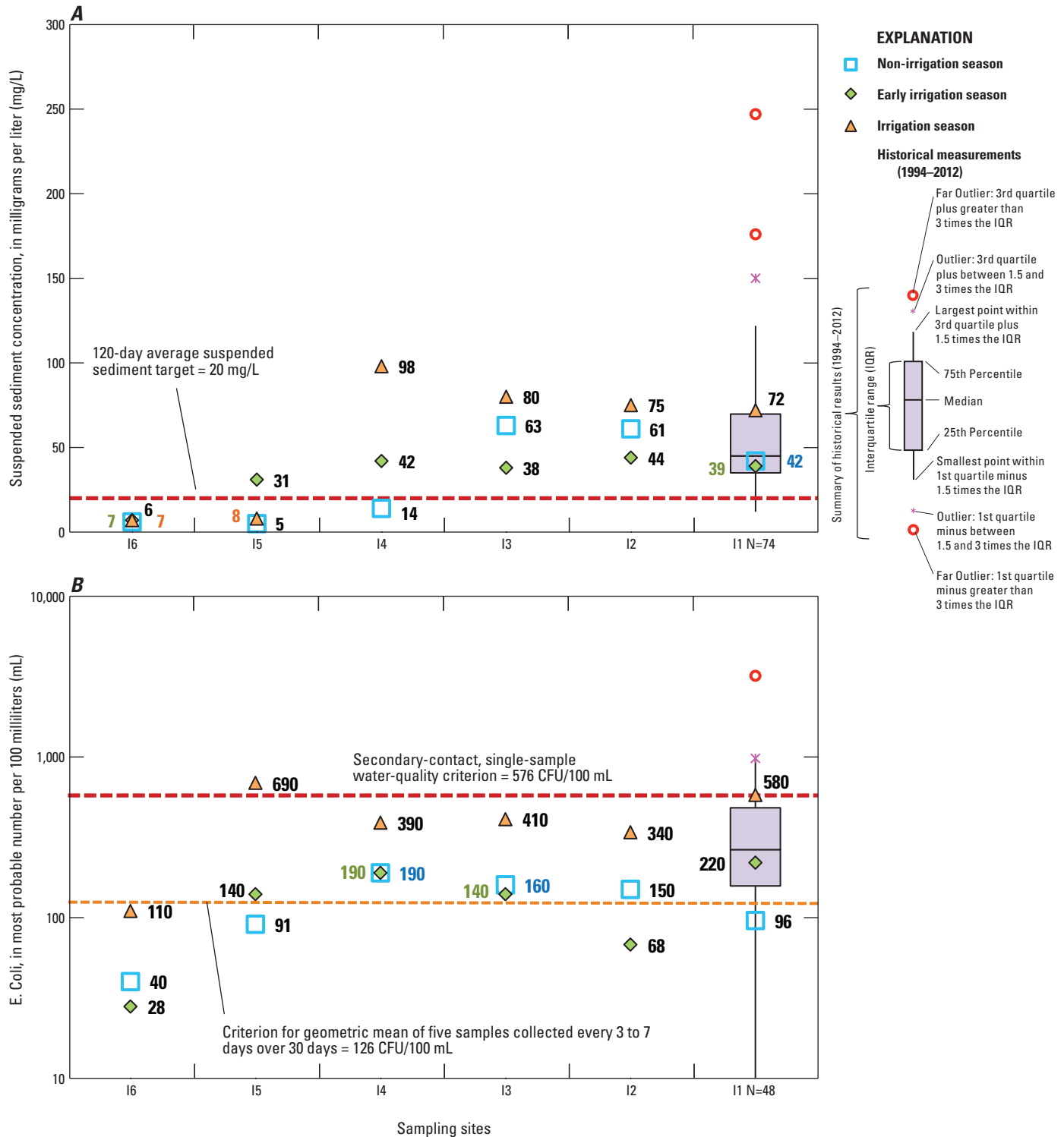
Figure 10. (A) Suspended-sediment concentrations and (B) Escherichia coli ( E. Coli ) values in samples collected from Indian Creek during 2010 compared with historical results (1994–2012) from Indian Creek at the mouth (site I1), southwestern Idaho. Locations of sites are shown in figure 1B . (N, number of samples).
