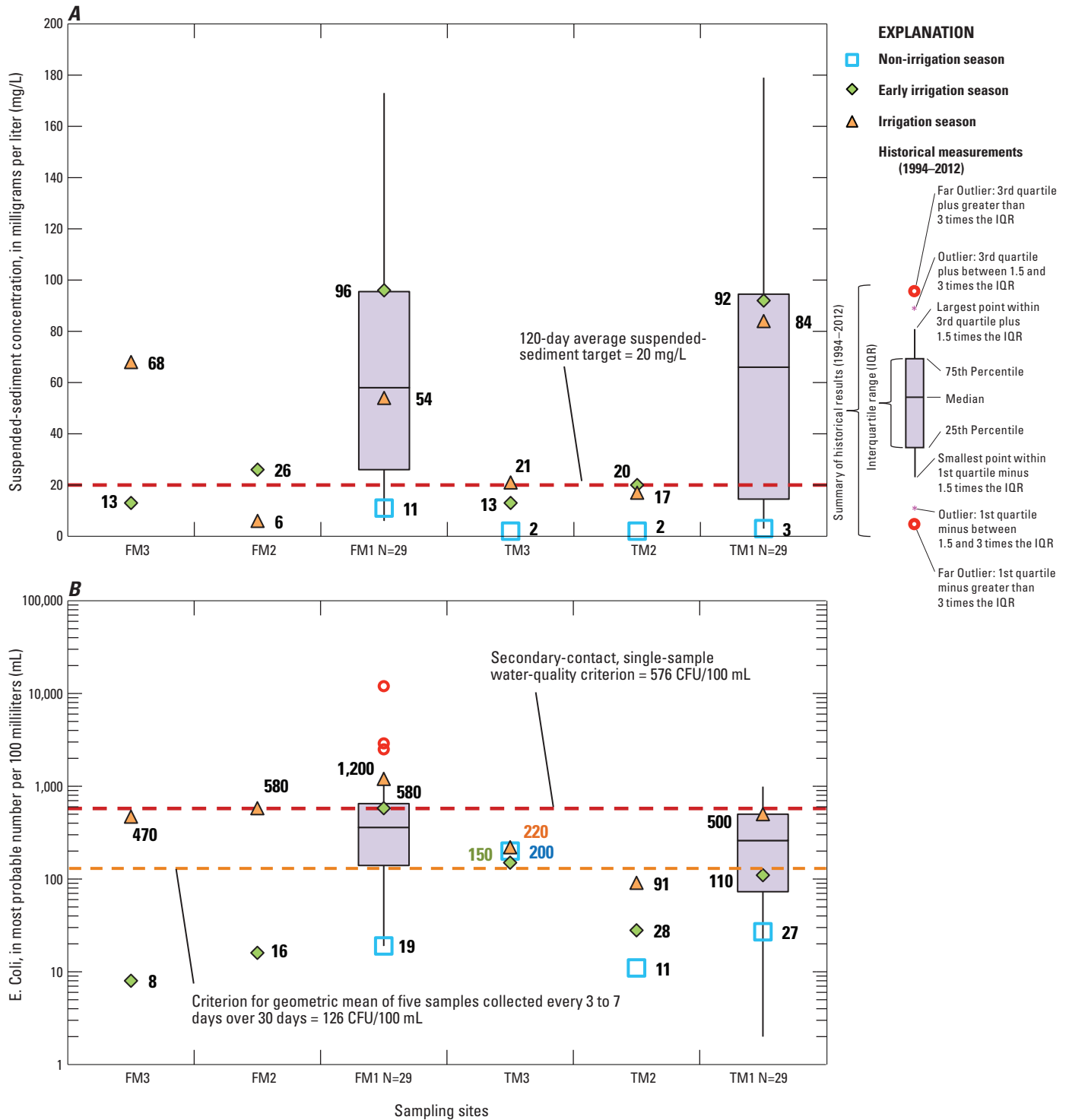
Figure 6. (A) Suspended-sediment concentrations and (B) Escherichia coli ( E. coli ) values in samples collected from Fivemile and Tennile Creeks during 2008 and 2009 compared with historical results (1994–2012) from Fivemile and Tennile Creeks at Franklin Road (sites FM1 and TM1), southwestern Idaho. Locations of sites are shown in figure 1B . (N, number of samples).
