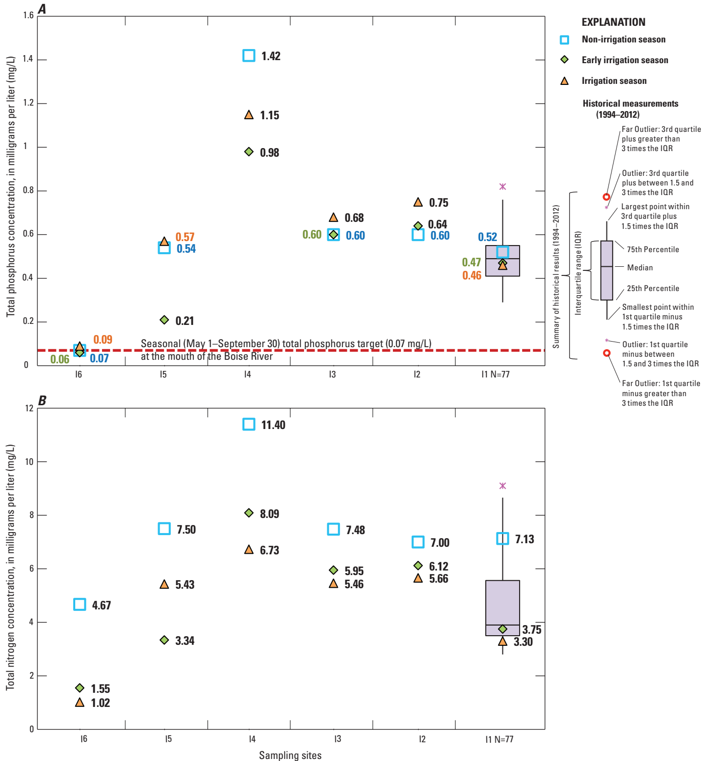
Figure 8. (A) Total phosphorus and (B) total nitrogen concentrations in samples collected from Indian Creek during 2010 compared with historical concentrations (1994–2012) in Indian Creek at the mouth (site I1), southwestern Idaho. Locations of sites are shown in figure 1B . (N, number of samples).
