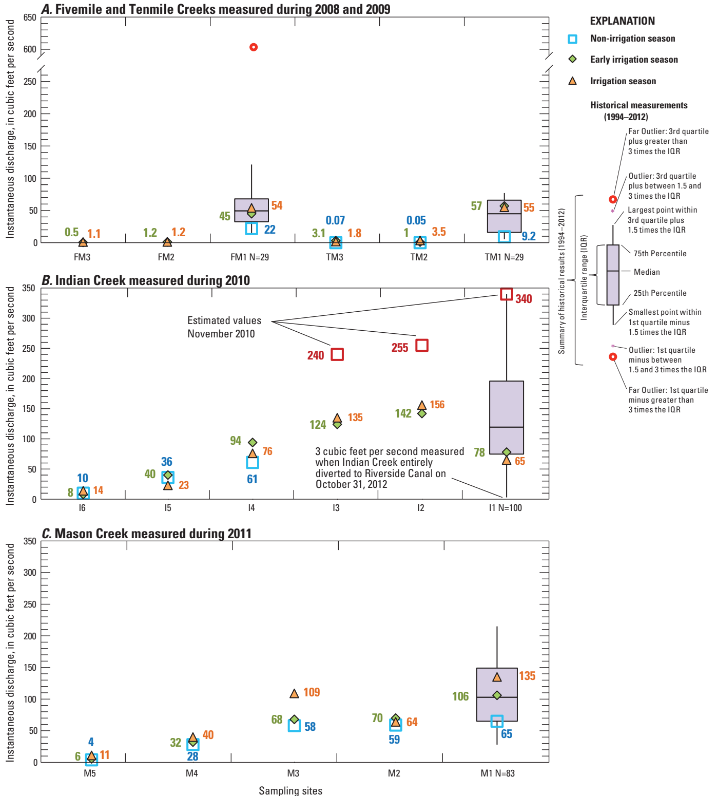
Figure 3. Instantaneous discharge from measurements in selected tributaries to the lower Boise River compared to historical discharge measurements near the mouth of each tributary (1994–2012), southwestern Idaho. (A) Discharge measured in Fivemile and Tenmile Creeks during 2008 and 2009 compared to historical discharge measured at sites FM1 and TM1 (1994–2012); (B) Discharge measured in Indian Creek during 2010 compared to historical discharge measured at site I1 (1994–2012); and (C) Discharge measured in Mason Creek during 2011 compared to historical discharge measured at site M1 (1994–2012). (N, number of samples).
