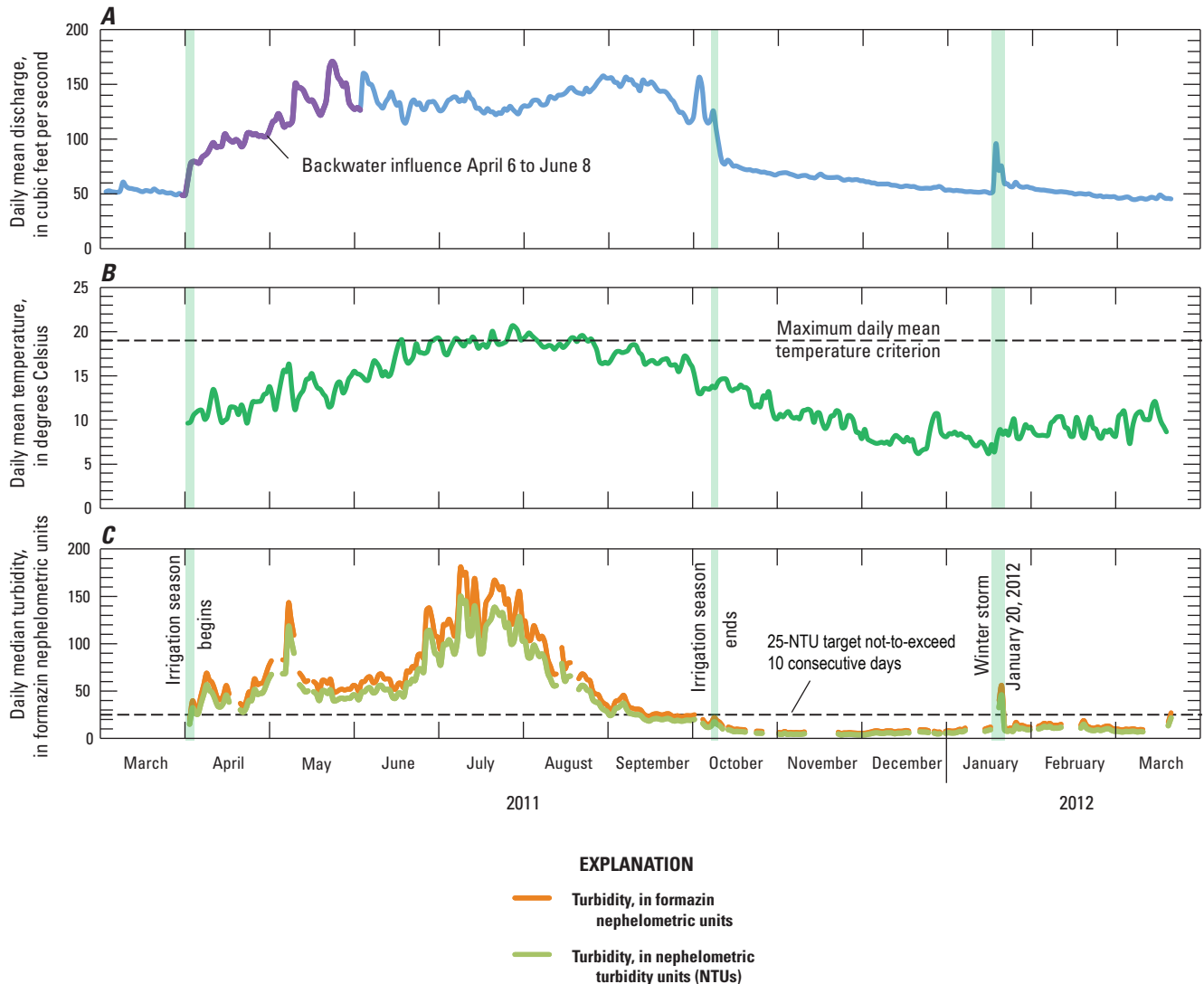
Figure 14. Daily mean values for computed (A) discharge and (B) water temperature, and daily median values for (C) turbidity at Mason Creek near Caldwell, Idaho, March 2011–March 2012..
