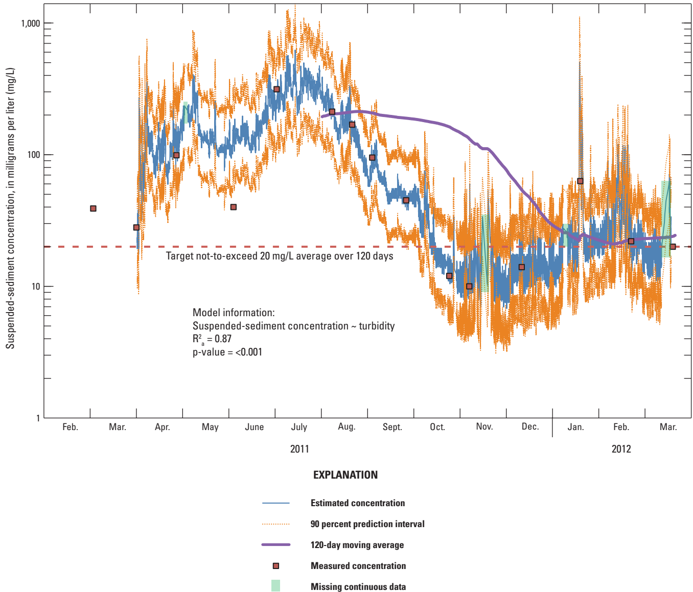
Figure 18. Estimated suspended-sediment concentrations based on a surrogate model developed for Mason Creek near Caldwell (site M1), Idaho, March 2011–March 2012.
