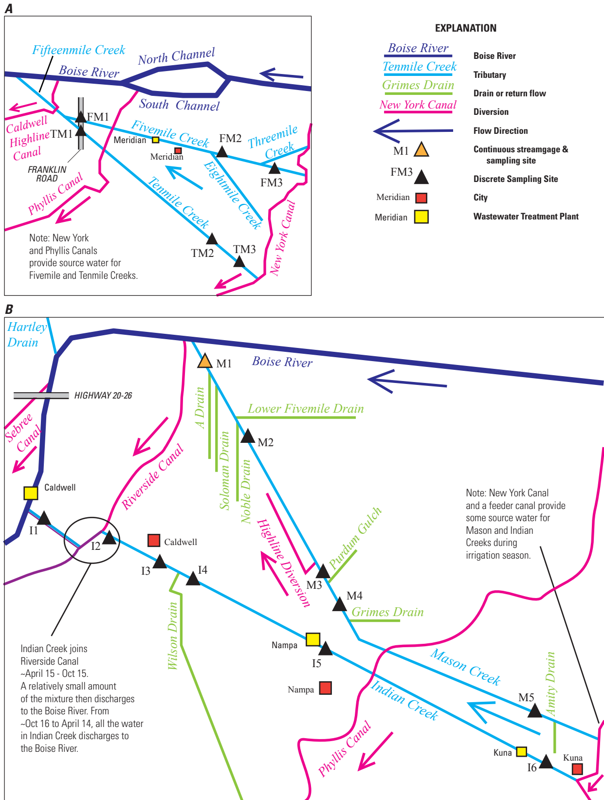
Figure 2. Fivemile, Tenmile, Mason, and Indian Creeks, lower Boise River watershed, southwestern Idaho.
