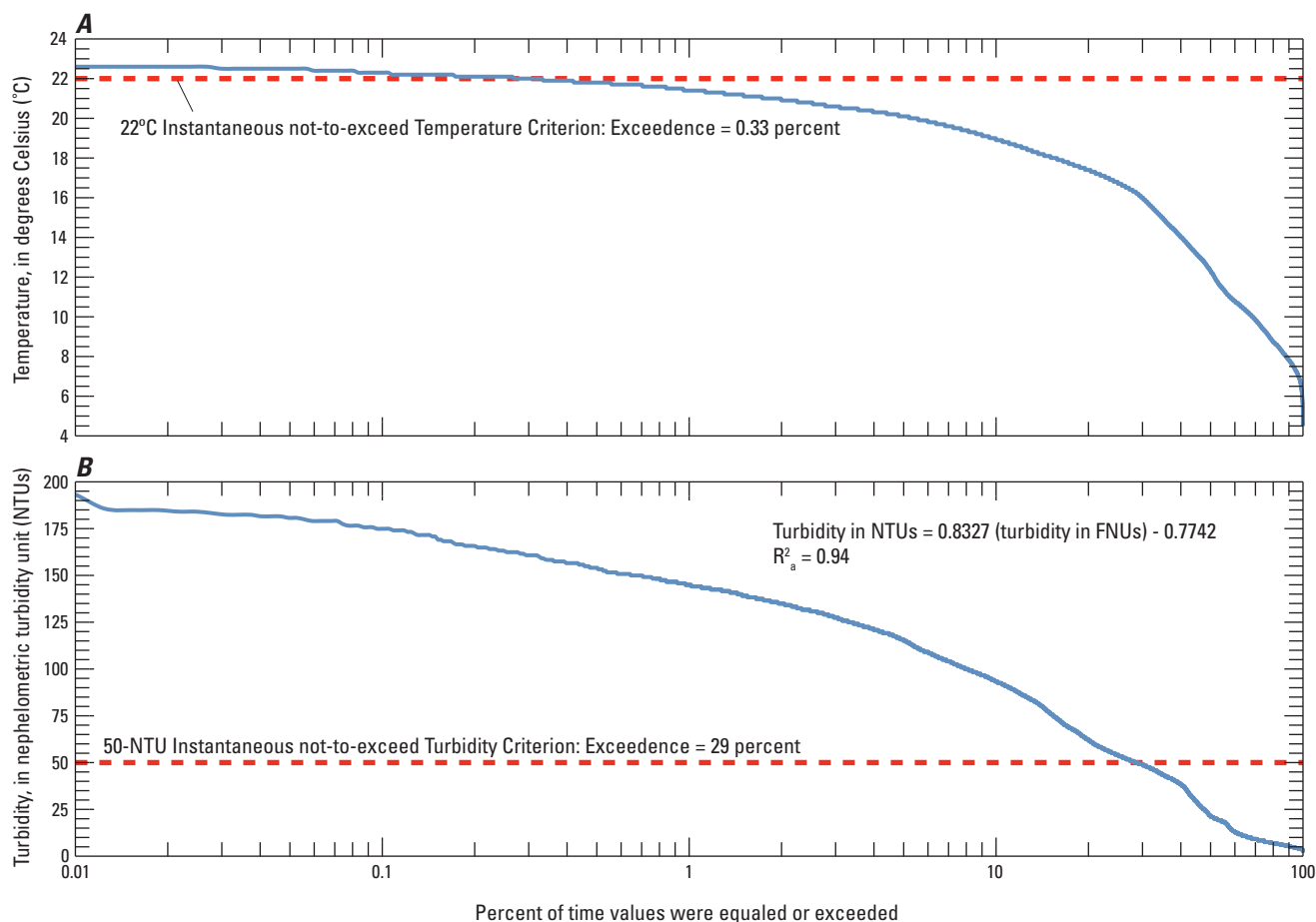
Figure 15. Exceedence curves for 15-minute values of (A) temperature and (B) turbidity in Mason Creek near Caldwell, Idaho, April 2011–March 2012.
