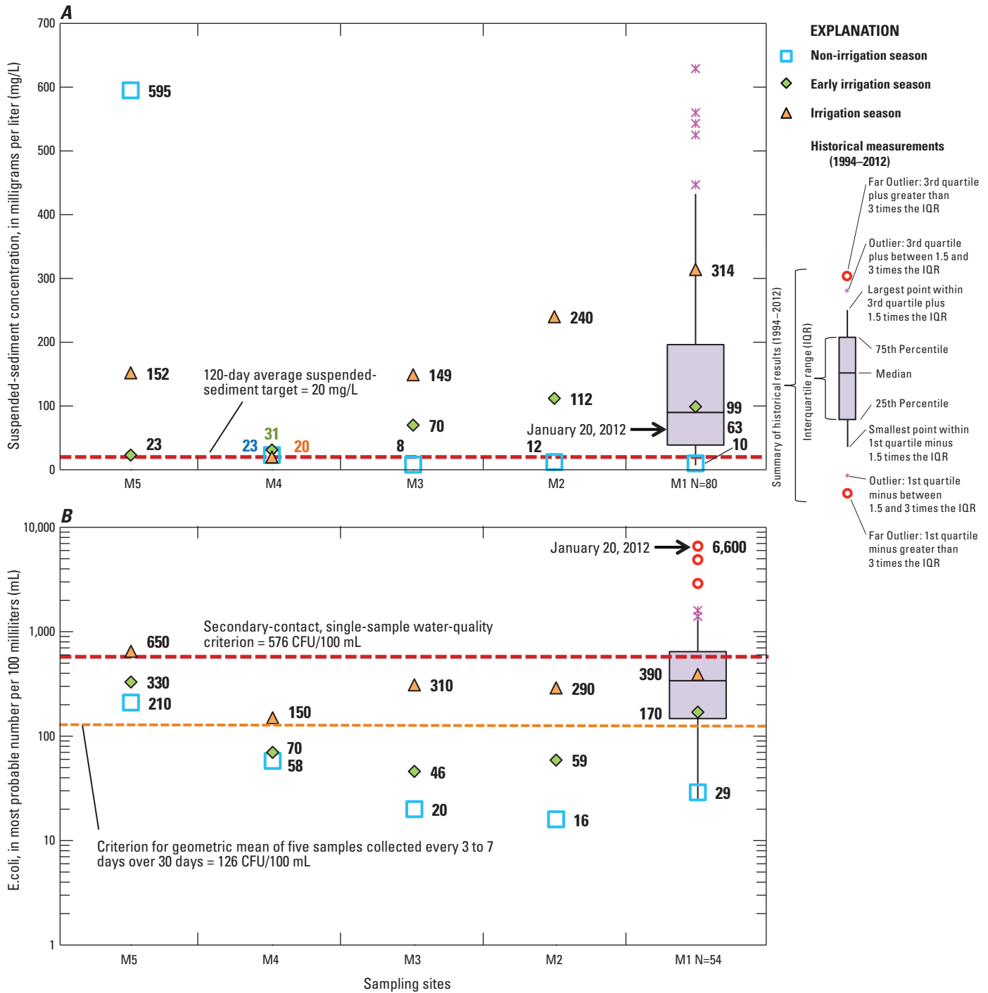
Figure 13. (A) Suspended-sediment concentrations and (B) Escherichia coli ( E. coli ) values in samples collected from Mason Creek during 2011, compared with historical results (1994–2012) from Mason Creek near Caldwell (site M1), southwestern Idaho. Locations of sites are shown in figure 1B . (N, number of samples).
