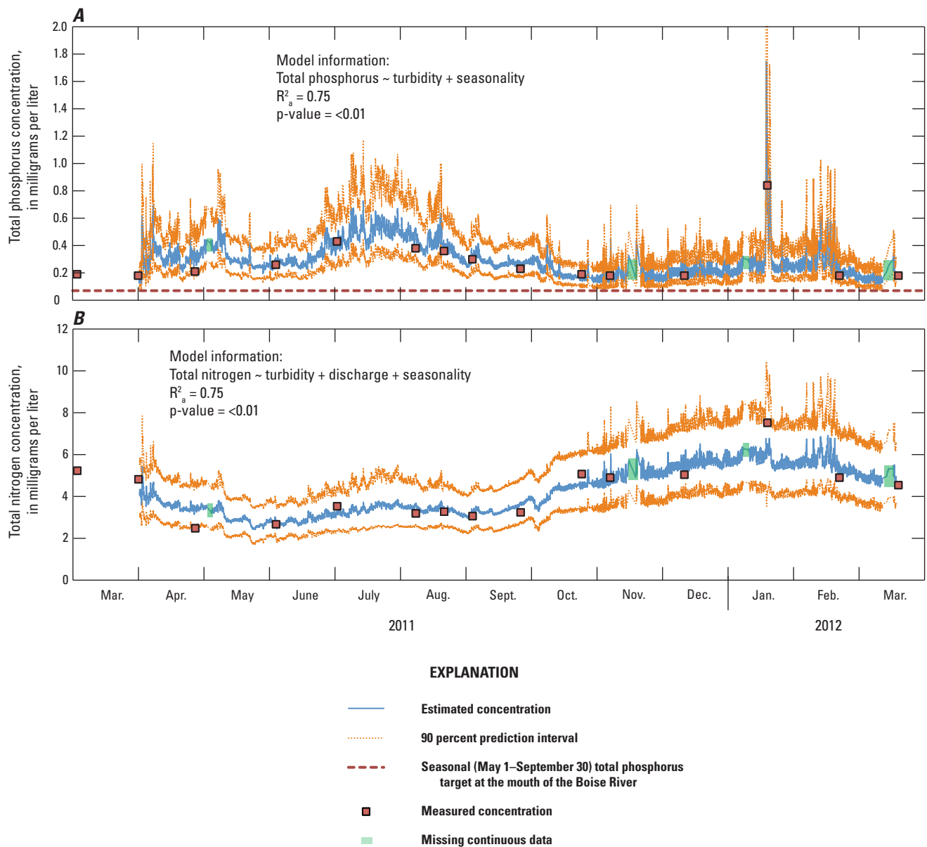
Figure 17. Estimated (A) total phosphorus and (B) total nitrogen concentrations based on surrogate models developed for Mason Creek near Caldwell (site M1), Idaho, March 2011–March 2012.
