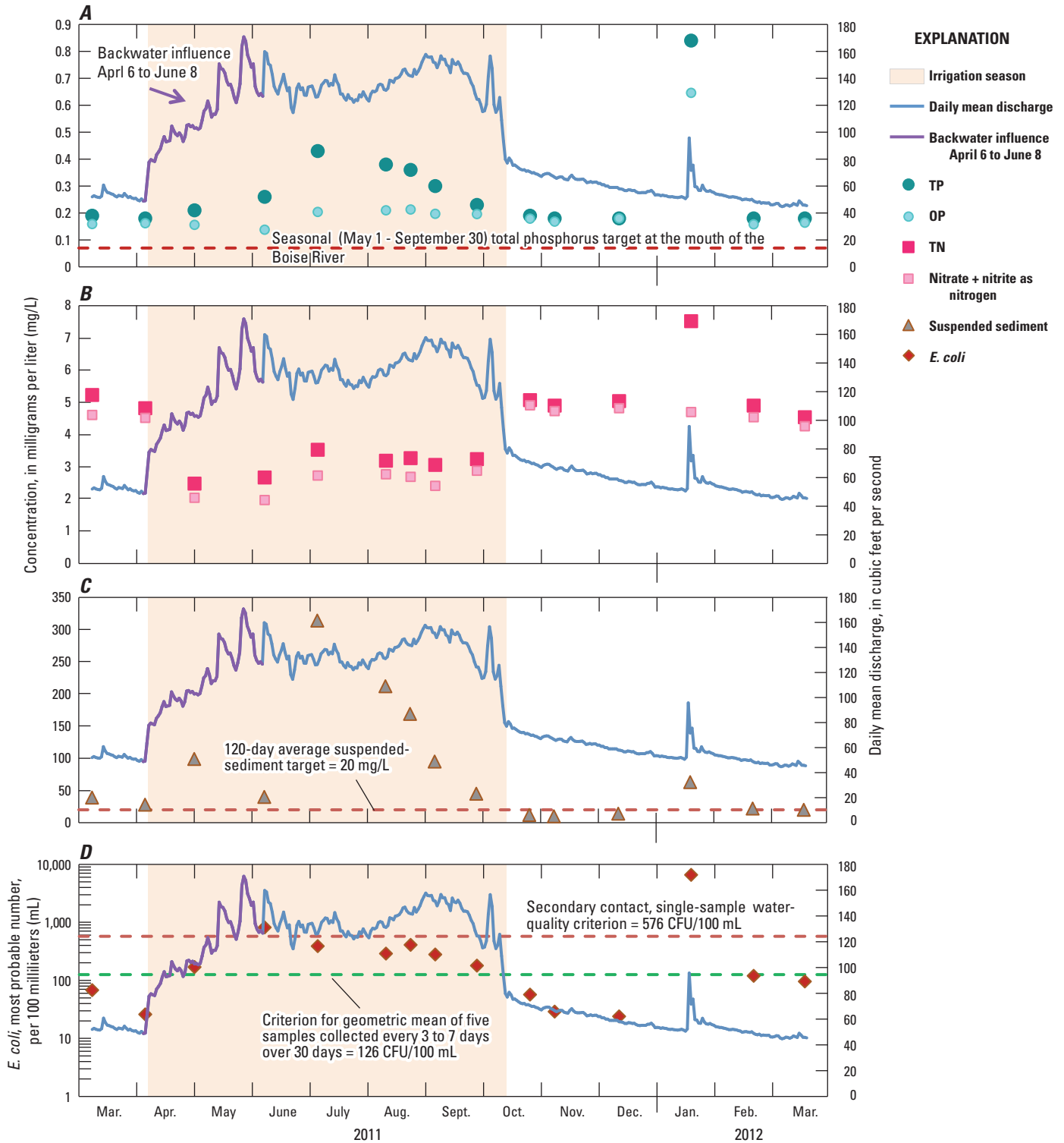
Figure 16. Concentrations of (A) phosphorus, (B) nitrogen, (C) suspended sediment, and (D) Escherichia coli ( E. coli ) in samples collected from Mason Creek near Caldwell (site M1), Idaho, March 2011–March 2012.
