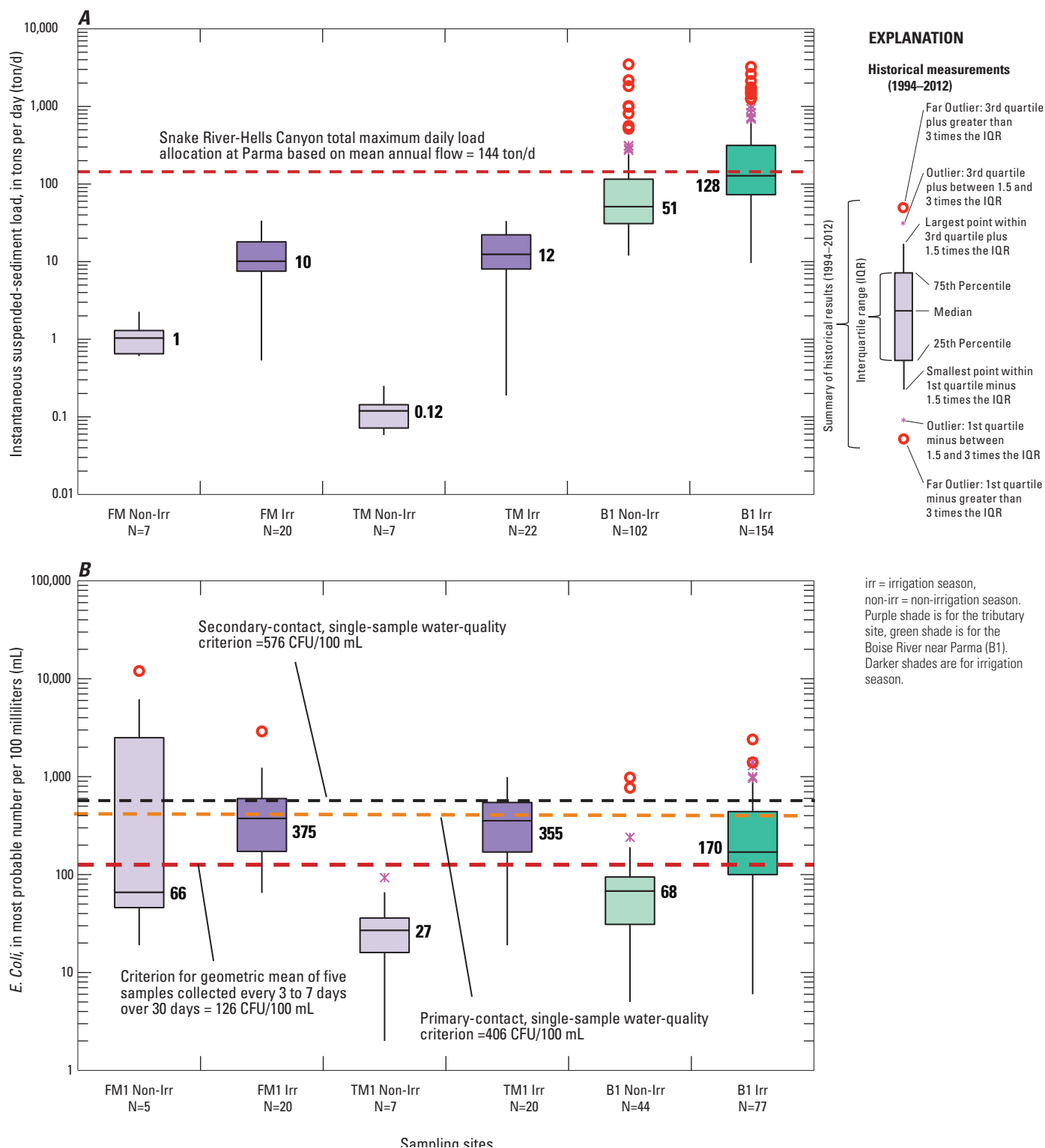
Figure 7. Historical instantaneous (A) suspended-sediment loads and (B) Escherichia coli ( E. coli ) values in irrigation and non-irrigation seasons in Fivemile and Tenmile Creeks (sites FM1 and TM 1) (1994–2012) and the Boise River near Parma (site B1) (1969–2012), southwestern Idaho. Locations of sites are shown in figure 1B . (N, number of samples).
