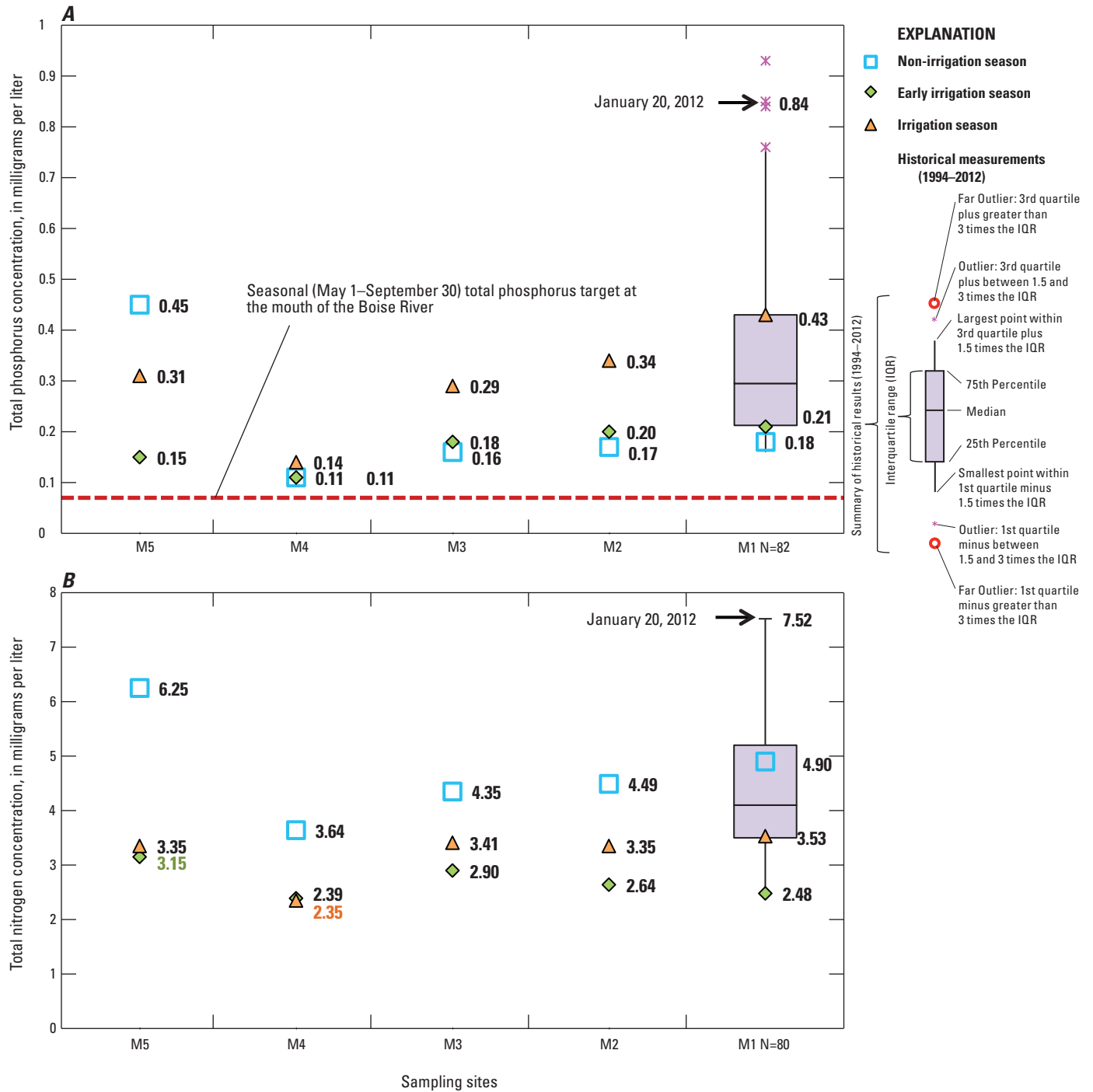
Figure 12. (A) Total phosphorus and (B) total nitrogen concentrations in samples collected from Mason Creek during 2011, compared with historical concentrations (1994–2012) from Mason Creek near Caldwell (site M1), southwestern Idaho. Locations of sites are shown in figure 1B . (N, number of samples).
